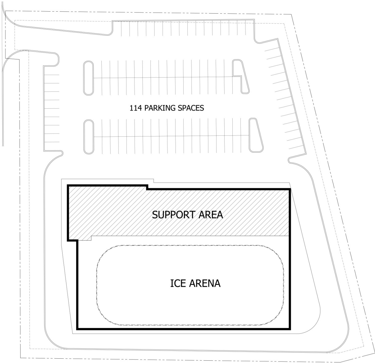
A PROPOSED THIRD ICE SHEET BUILDING LAYOUT - OPTION NO. 1 0 8' 16' 32'
